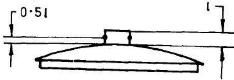
Fig. 4D Points For Temperature Measurement - Knob
