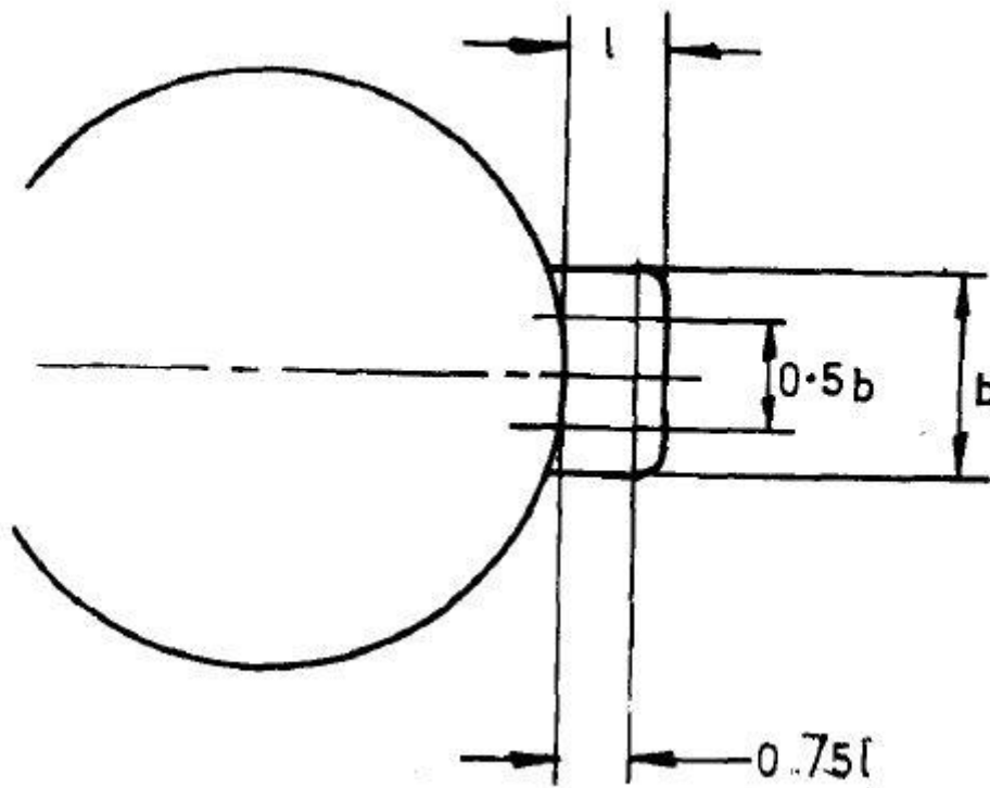
Fig. 4B Points for Temperature Measurement - Solid Flange Handle
