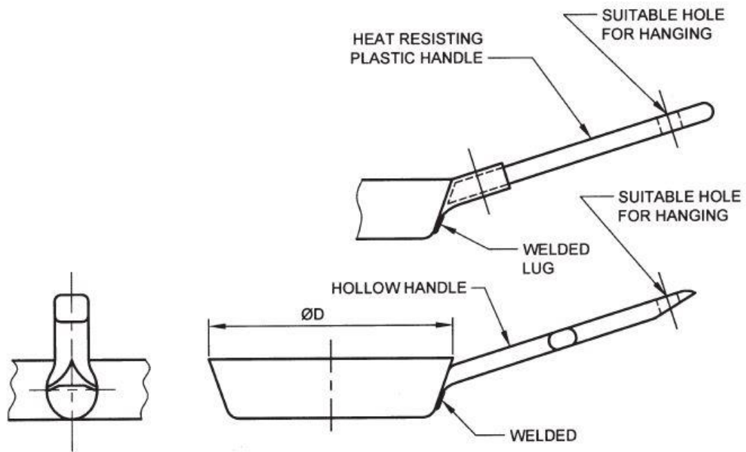
Fig. 8 Frying-Pan
