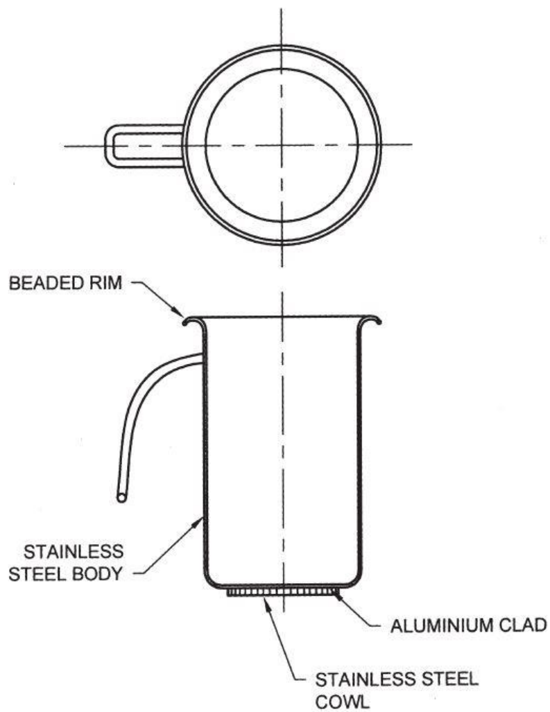
Fig. 16 Cassrole with Cladded Base
